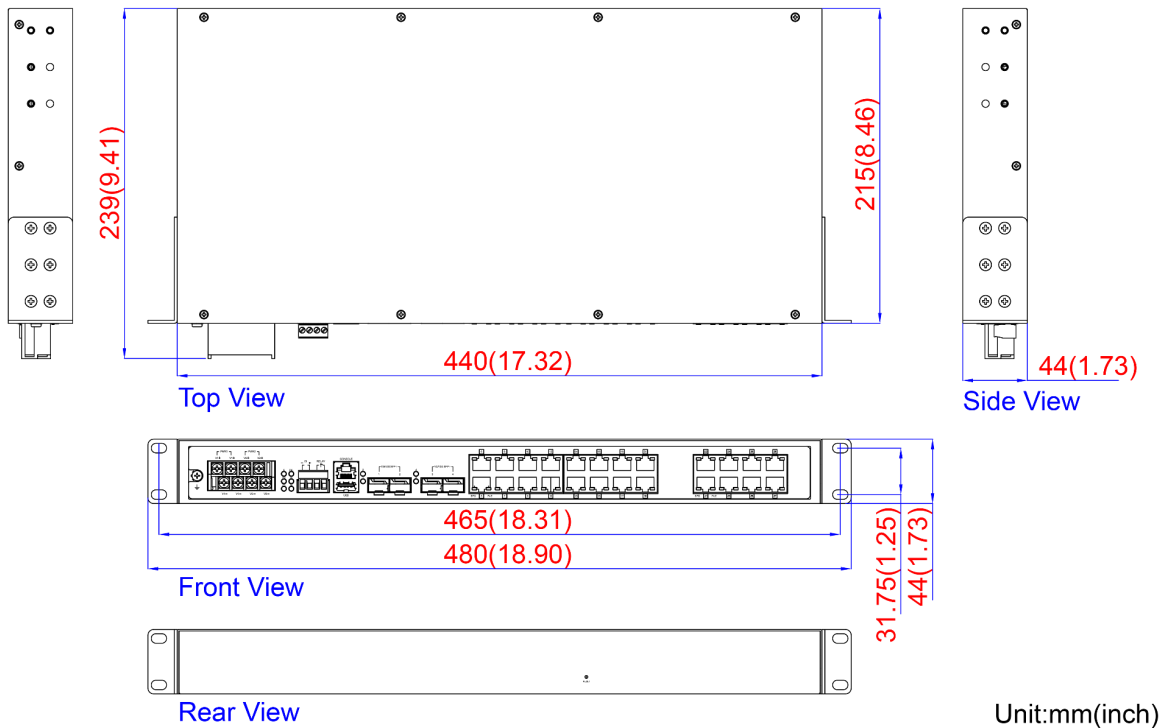
Figure 2.1 - Physical Dimensions
