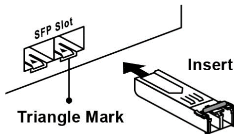
Figure 2.4 - Transceiver to the SFP Module
