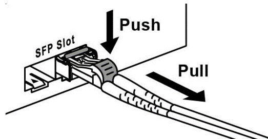
Figure 2.7 - Remove LC Connector
